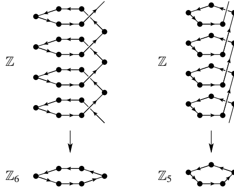
FIGURE 1. The universal covering of the quandle Q_{6,5}
