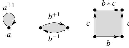
FIGURE 2. Elementary homotopies for paths in P(Q)
